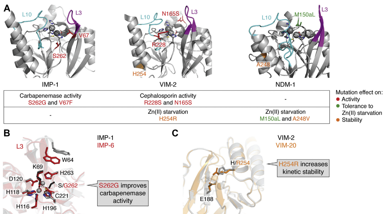
Figure 4. A, key mutations and evolutionary traits in the main families of acquired MBLs: IMP-1, VIM-2, and NDM-1. Figures were rendered with PyMol based on the PDB IDs 4C1G, 4N2Q, and 3SPU, respectively. The active-site loops L10 and L3 are shown in cyan and magenta, respectively; the metal ligands as sticks, and the Zn(II) ions as spheres. The mutational “hot spots” are indicated in different colors according to their impact on catalytic activity (red) (79, 130, 139) or in the tolerance against Zn(II) starvation by improving metal binding (green) or the kinetic stability (orange) (73, 74, 79). B, a conformational change in loop L3 introduced by substitution S262G in IMP improves carbapenemase activity. The interaction between S262 and K69 marked with black dashes in IMP-1 (gray structure) is disrupted by the substitution in IMP-6 (red; PDB: 6LVJ). C, the substitution H254R increases the kinetic stability of VIM-20 (PDB: 6OP6) by the formation of a salt bridge between R254 and E188. IMP-1, imipenemase 1; MBL, metallo- \beta -lactamase; NDM-1, New Delhi metallo- \beta -lactamase 1; PDB, Protein Data Bank; VIM-2, Verona imipenemase 2.
