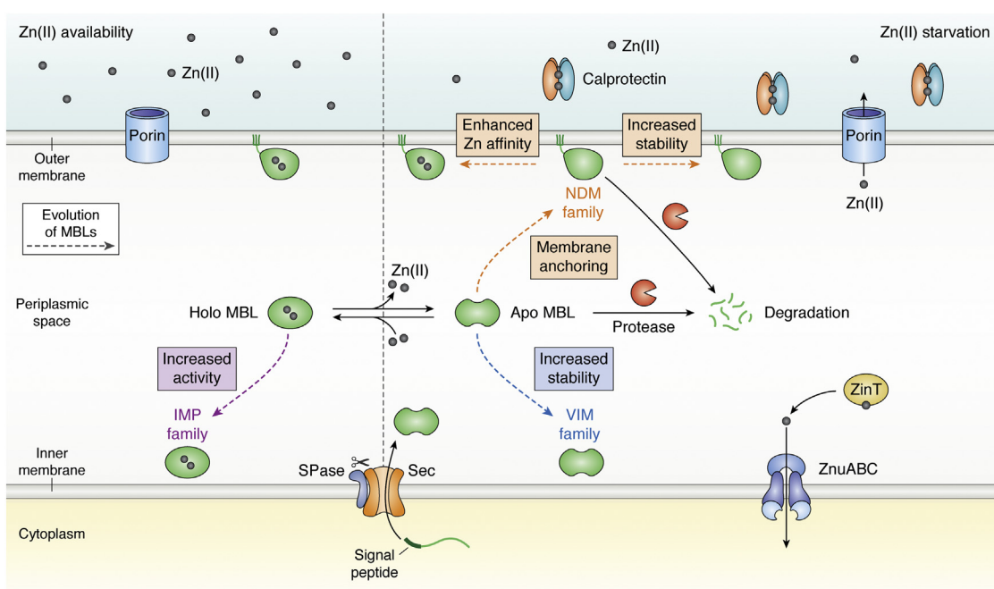
Figure 2. Mechanisms of MBL evolution. Periplasmic Zn(II) levels depend on the passive diffusion through porins in Escherichia coli . In the presence of Zn(II), represented by gray spheres (left panel), the external concentration is in equilibrium with periplasmic Zn(II) levels (62, 63), and MBLs bind the cofactor and hydrolyze \beta -lactams. The dashed arrows highlight the different mechanism of MBL evolution (79, 130, 139). IMP families have evolved increasing their activity in response of antibiotic evolutionary pressure. When the innate immune response is active (right panel), neutrophils secrete calprotectin (CP) that chelates Zn(II) ions (43), reducing the periplasmic Zn(II) levels and activating expression of the Zn(II) uptake mechanisms to the E. coli cytosol (ZnuABC system and ZinT chaperone). MBLs lose the Zn(II) cofactor leading to formation of apo-MBLs. The nonmetallated form is susceptible to degradation in the periplasm by proteases (shown as Pac-Man-like orange objects) (44). Different mechanisms of evolution are indicated with dashed arrows of different colors, such as outer membrane anchoring (44), stabilization toward degradation, or enhancement of the Zn(II) affinity (15, 73). IMP, imipenemase; MBL, metallo- \beta -lactamase; SPase, signal peptidase.
