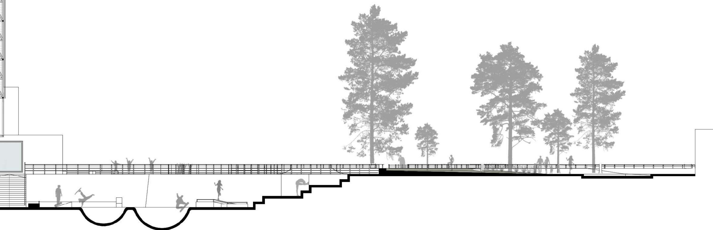
CORTE GENERAL 1-1
