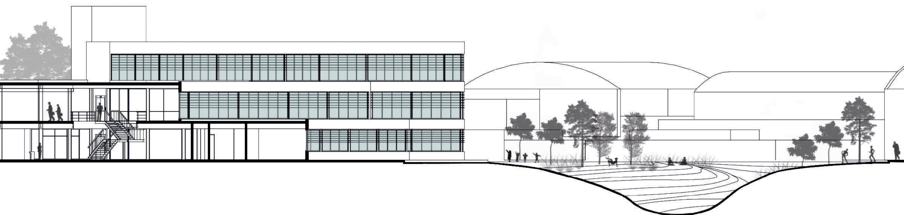
CORTE GENERAL 2-2
