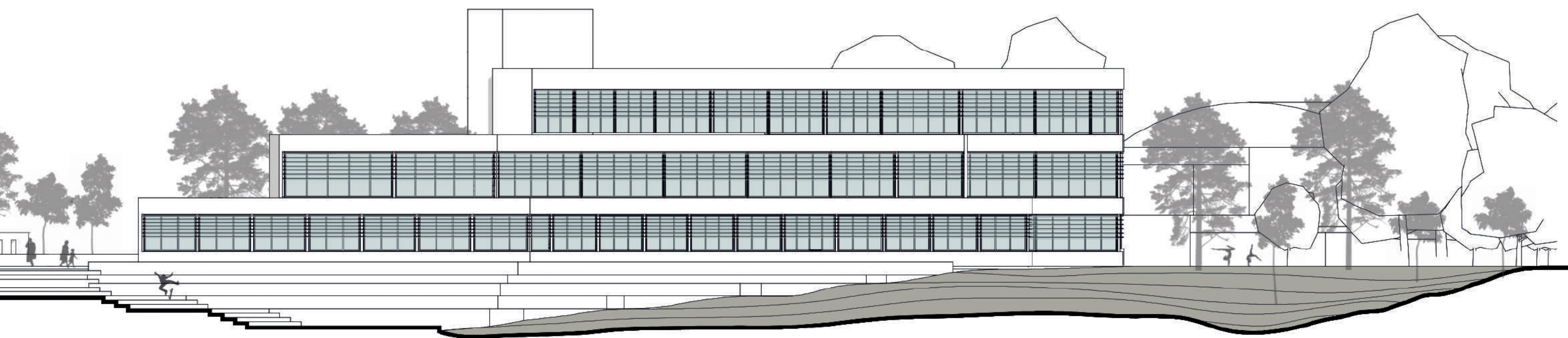
CORTE GENERAL 4-4
