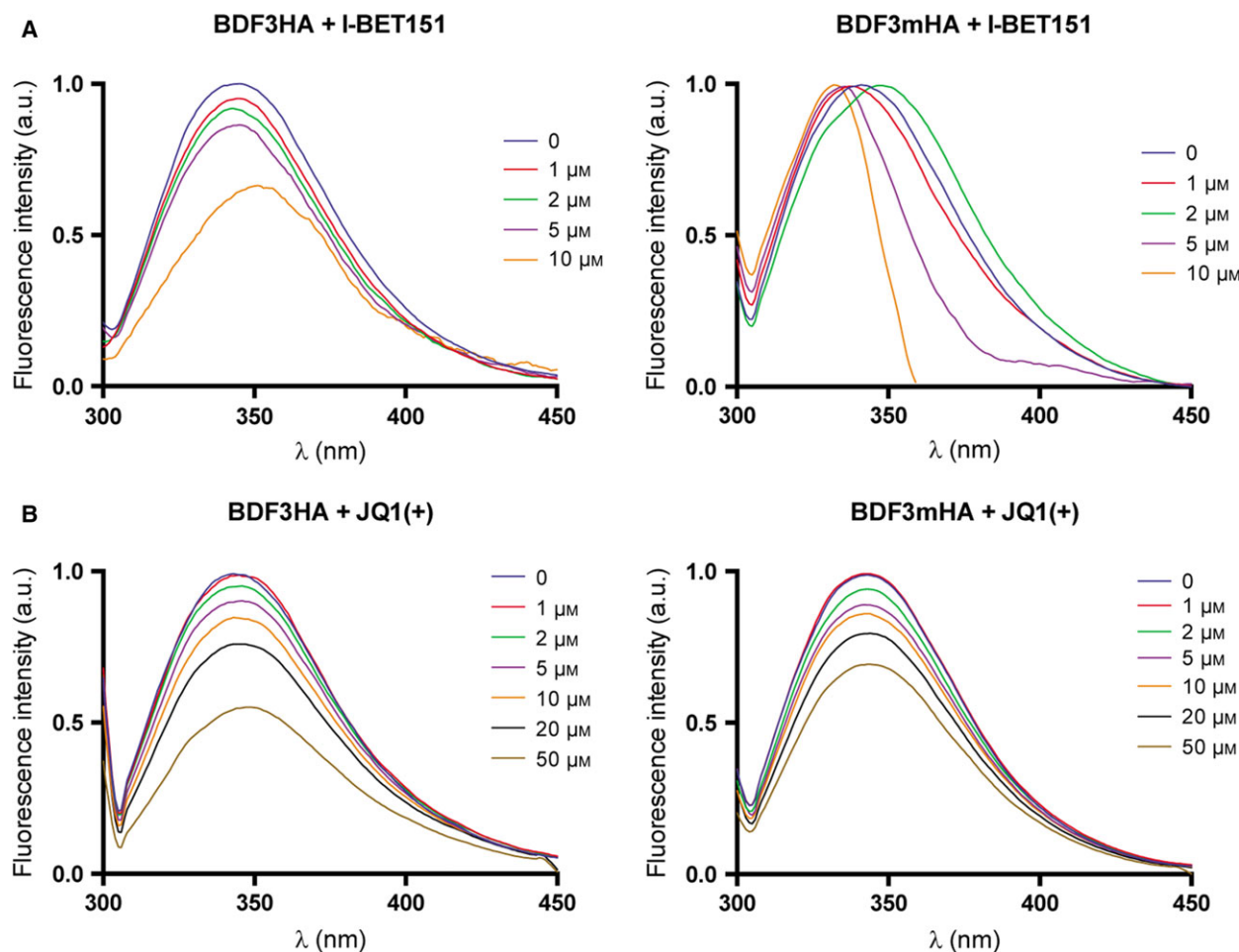
Fig. 5. Bromodomain inhibitors interact with recombinant TcBDF3HA and TcBDF3mHA. Fluorescence spectra of TcBDF3HA and TcBDF3mHA (5 μM) with an increasing amount of I-BET151 (A) and JQ1(+) (B). λ ex = 295 nm.
