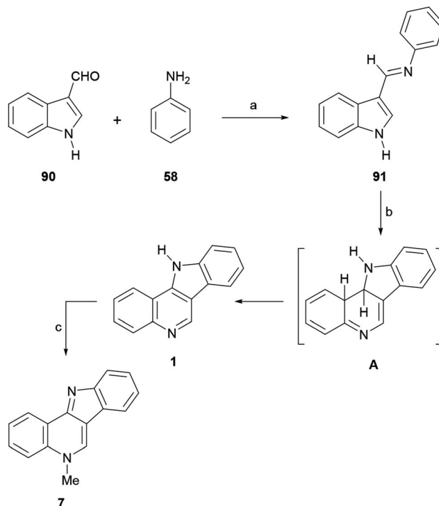
Scheme 21 Reactions and conditions: (a) AcOH_{gl} , reflux, 3 h (85%); (b) (1) h\nu (254 nm), PhH-MeOH , rt, 2 : 1; (2) I_2 , 48 h (67% overall); (c) Me_2SO_4 , MeCN , reflux, 6 h, K_2CO_3 (83%).
