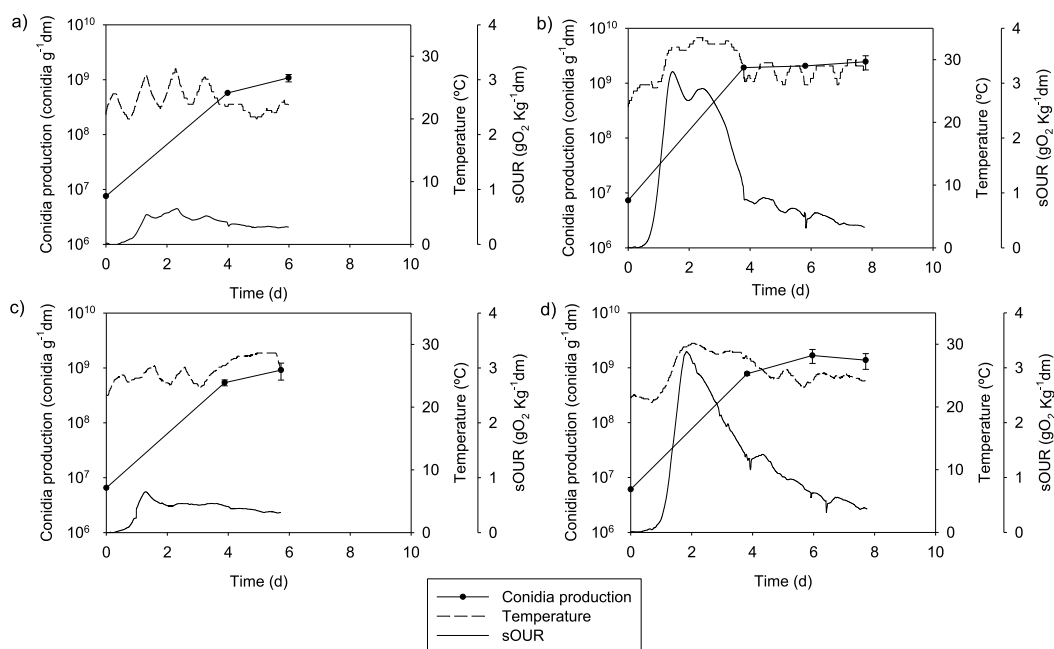
Fig. 3. TH profiles (conidia production, sOUR and mean temperature) obtained in packed bed bioreactors. a) 1.5 L rice husk; b) 1.5 L beer draf; c) 22 L rice husk and d) 22 L beer draf.
