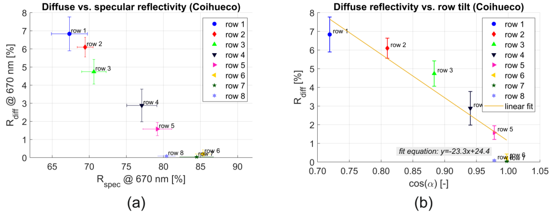
Figure 6. (a) Negative correlation between quantities R_{\text{diff}} and R_{\text{spec}} at the CO5 telescope. As seen in (b) the diffuse reflectance depends on the tilt of the row. The results were obtained at 670 nm and an angle of incidence of 25^\circ according to the specification of the \mu Scan device. These results are based on measurements taken in November 2024 (96 months from cleaning). Mean values and standard deviations were calculated from measurements at five different positions on each segment.
