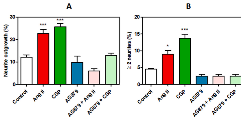
Fig. 6. Tyrostatin AG879, a TrkA inhibitor, prevents neurite outgrowth induced by Ang II and CGP42112A. (A) SH-SY5Y cells were pre-treated with AG879 (0.6 \mu M, 40 min), stimulated with CGP42112A, allowed to differentiate for 3 days and neurite outgrowth was quantified. Values represent mean \pm S.E.M (n = 3), ***p < 0.001 vs. control. (B) Graph showing the percentage of cells exhibiting 2 or more neurites. Values represent means \pm S.E.M (n = 3). *p < 0.05, ***p < 0.001 vs. control.
