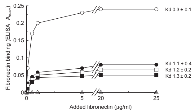
Fig. 8. Kinetics and saturability of the binding of B. subtilis and Gram-positive pathogens to fibronectin. Microtitre plates were coated with the corresponding bacterial strains and incubated with increasing amounts of fibronectin for 2 h at 37°C. Bound protein was detected with anti-fibronectin monoclonal antibody and mouse anti-IgG peroxidase-conjugated and quantified with TMB one-step substrate system. The results are representative of three experiments performed by triplicate. The apparent dissociation constants (Kd) \pm S.E.M. (indicated on the figure) were calculated (in nM) using the computer program Grafit 4 (see Experimental procedures for details). Symbols: ( \circ ) RG4365 (wild-type B. subtilis ); ( \bullet ) BBB ( S. aureus ); ( \square ) BBB ( E. faecalis ); ( \blacksquare ) ATCC7644 ( L. monocytogenes ); ( \triangle ) RG4376 ( yloA B. subtilis ).
