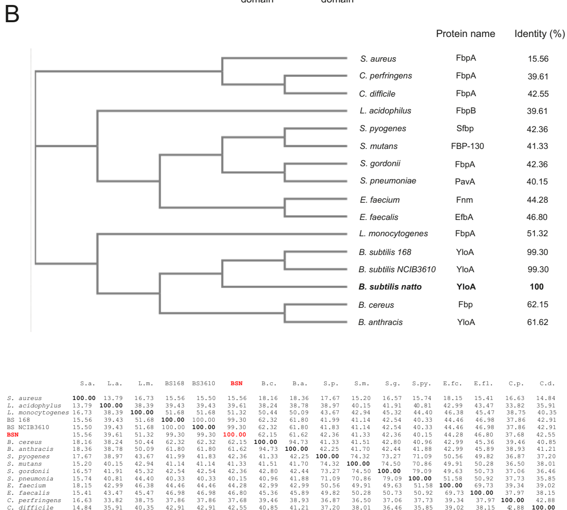
Fig. 4. Schematic representation and phylogenetic conservation of yloA .
