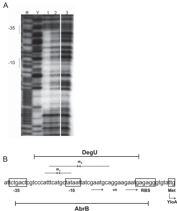
Fig. 7. AbrB- and DegU-recognized promoter regions of yloA . A. DNAase I footprinting analysis of AbrB binding to a DNA fragment of the strain RG4365 containing the yloA promoter region. Shown is the non-template strand labeled at its 3' end. Lanes: 1, 30 \mu M AbrB; 2, 9 \mu M AbrB; 3, no AbrB. Maxam-Gilbert purine (R) and pyrimidine (Y) sequencing ladders are shown for positioning reference. The putative -10 and -35 regions of the promoter are indicated by the vertical bars on the left. All binding reactions were performed at pH 8. B. Sequence of the yloA promoter region showing extends of AbrB- afforded protection from DNAase cleavage and the putative DegU- recognized binding sites (see text for details).
